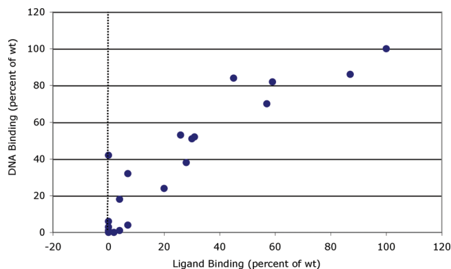
FIGURE 5: Correlation between [ 3 H]TCDD ligand binding and TCDD-dependent DNA binding of mAhRs containing mutations of selected residues within the LBD. Ligand binding to in vitro expressed wild-type or mutant AhR incubated with 4 nM [ 3 H]TCDD and unprogrammed reticulocyte lysate (nonspecific binding control) was assessed using hydroxyapatite binding, and DNA binding (formation of the AhR-ARNT-DRE complex) of in vitro expressed wild-type or mutant AhR and wt ARNT incubated with DMSO (control) or 20 nM TCDD was assessed by gel retardation analysis as described in Materials and Methods. The amount of [ 3 H]TCDD specific binding to and AhR-ARNT-DRE complex formation of each mutant AhR was expressed relative to that of wild-type AhR (100%), and the specific values are listed in Table 3.
