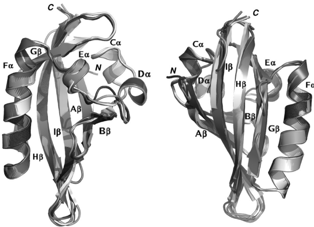
FIGURE 2: Cartoon representation of the modeled structures of the AhR LBDs from seven different species, structurally aligned with DALILite (36, 37) and shown in two different orientations.
