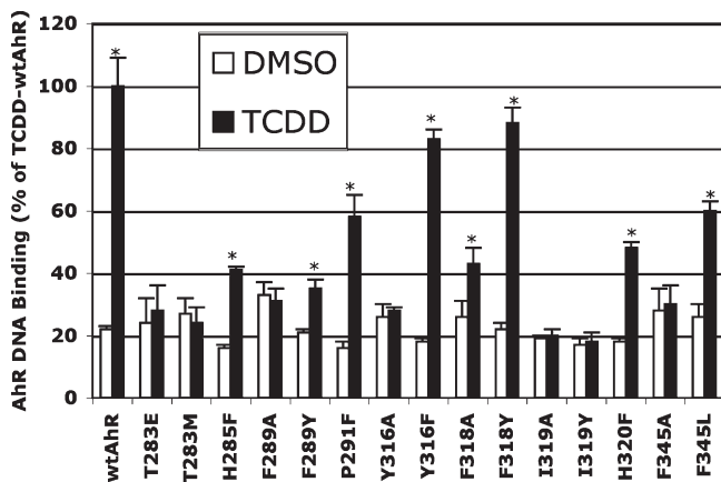
FIGURE 4: Effect of mutation of selected residues within the mAhR LBD on TCDD-dependent AhR DNA binding. In vitro expressed wild-type or mutant AhR and wt ARNT were incubated with DMSO (control) or TCDD, and formation of the AhR-ARNT-DRE complex was assessed by gel retardation analysis as described in Materials and Methods. Quantitation of the amount of AhR-ARNT-DRE complex was achieved by phosphorimager analysis, and the results are expressed as the mean ± standard deviation of multiple receptor preparations and gel retardation analyses ( n ≥ 3). The asterisk indicates that the values are significantly different from those of their respective DMSO control at p ≤ 0.05 as determined by a Student's t test. The amount of specific TCDD-inducible AhR-ARNT-DRE complex for each AhR determined after subtraction of the DMSO background is presented in Table 3.
